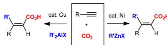
Scheme 2. CO 2 Insertion into Terminal Alkyne Using Organozinc and Organoaluminum
