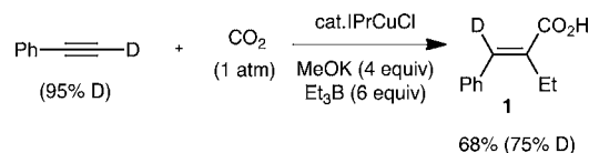
Scheme 4. Deuterium-Labeling Experiment for Cu-Catalyzed CO 2 Insertion of Phenylacetylene- d
