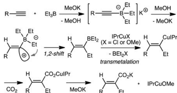
Scheme 5. Plausible Reaction Mechanism for Cu-Catalyzed \text{CO}_2 Insertion into Terminal Alkynes
